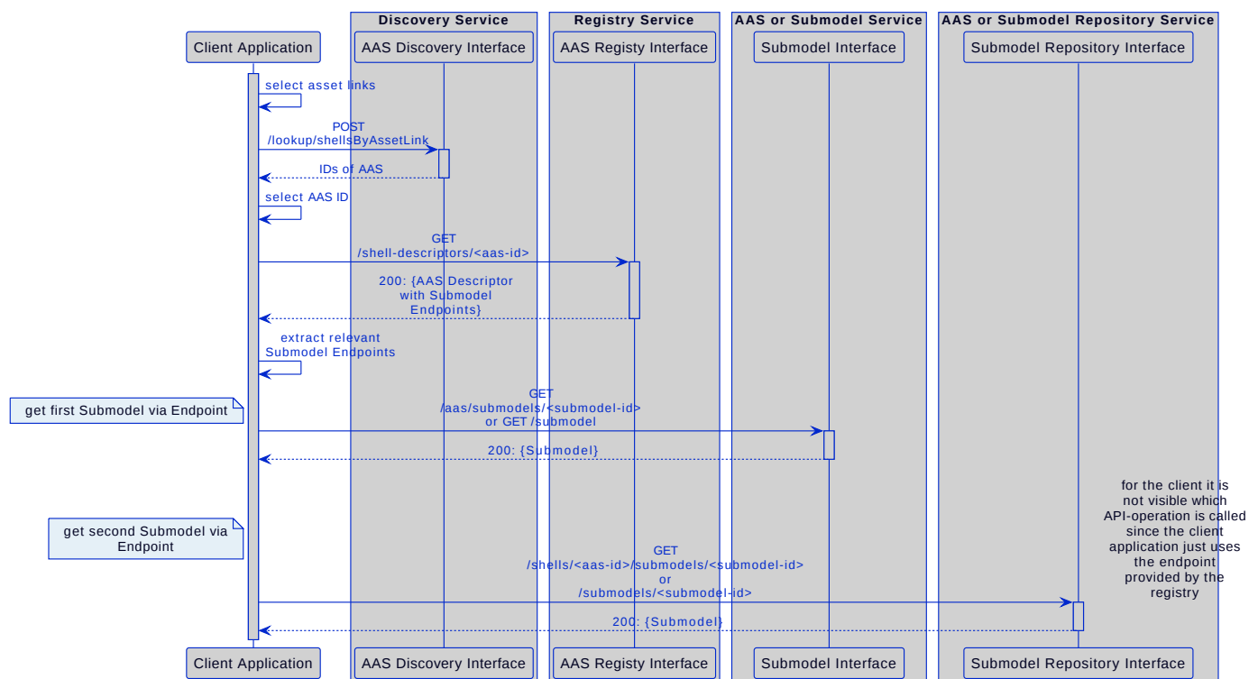
Figure 10. Interaction for Client Application using Submodel Endpoints
