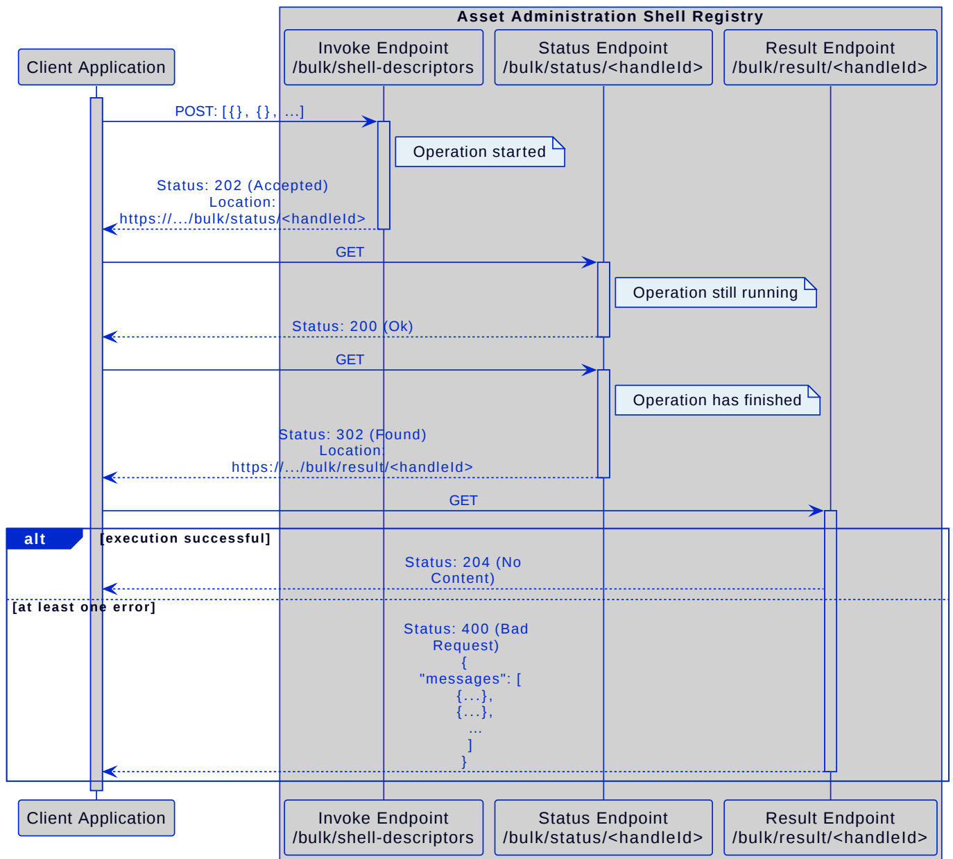
Figure 9. Sequence of a Bulk API Operation
