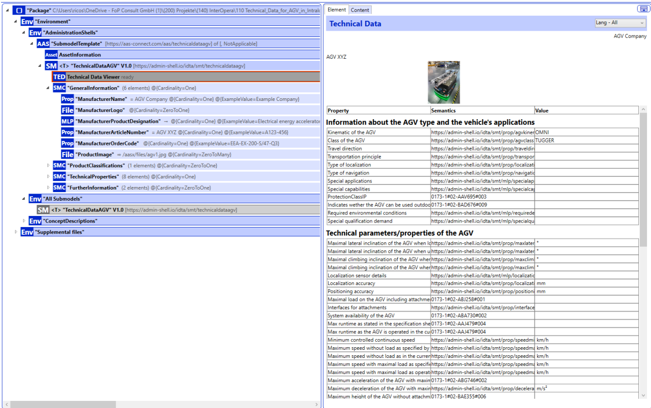
Figure 4: Screenshot of the Technical Data Viewer (specific plug-in of the Package Explorer)
