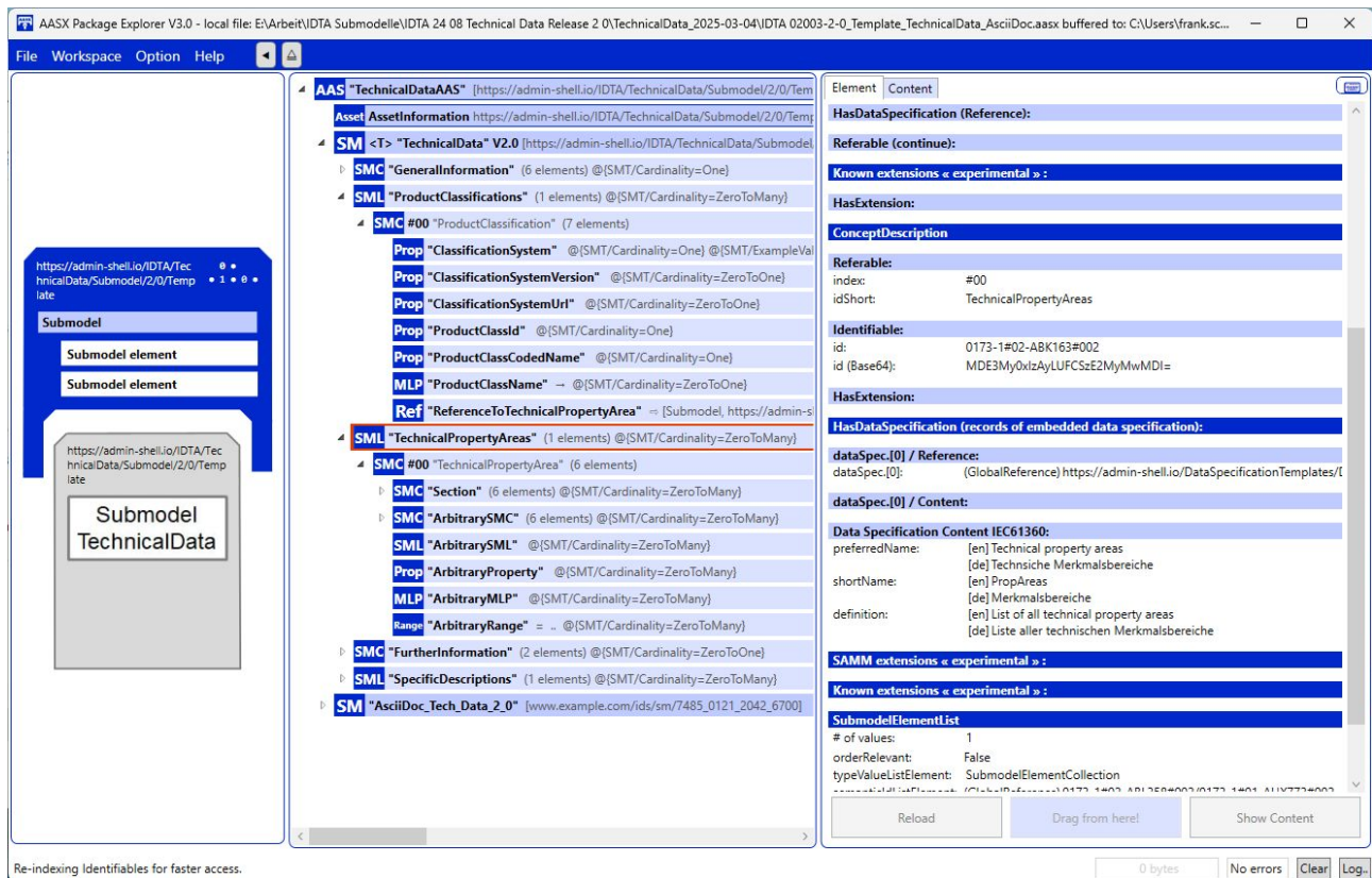
Figure 3. Exemplary presentation in an AAS user application
