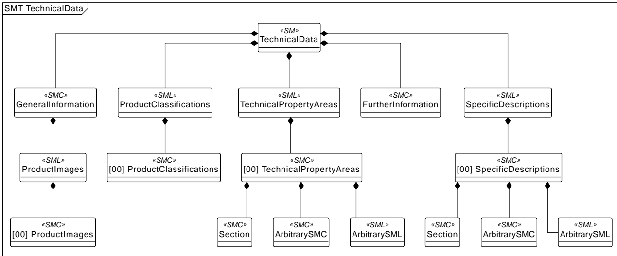
Figure 2. UML overview
