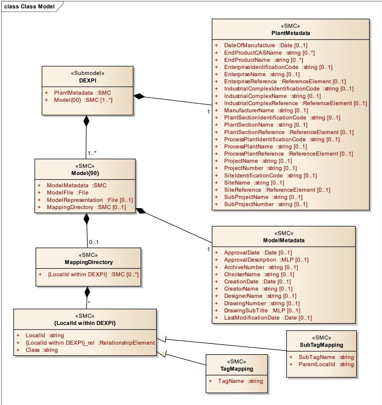
Figure 2: UML class diagram of the Submodel
