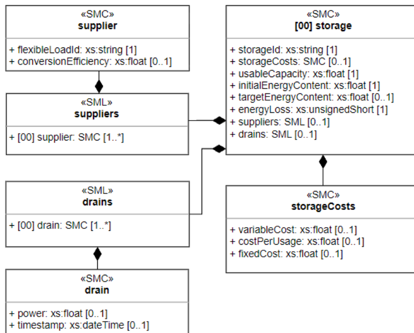
Figure 13 UML diagram of SMC [00] storage
