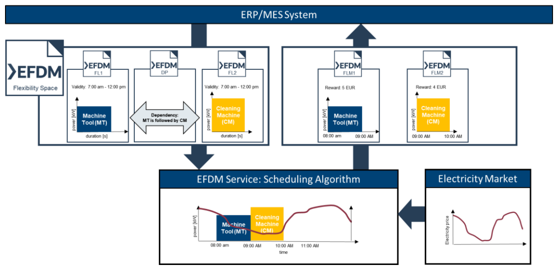
Figure 3 Using EFDM in the scheduling problem for optimal energy cost
