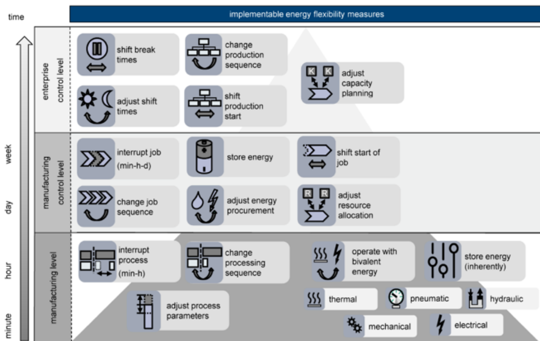
Figure 7 Exemplary flexibility measures described in VDI 5207 Part-1 [7]
