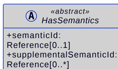
Figure 10. Metamodel of Semantic References ( HasSemantics )
