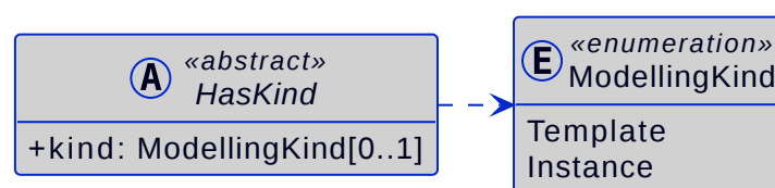
Figure 9. Metamodel of HasKind
