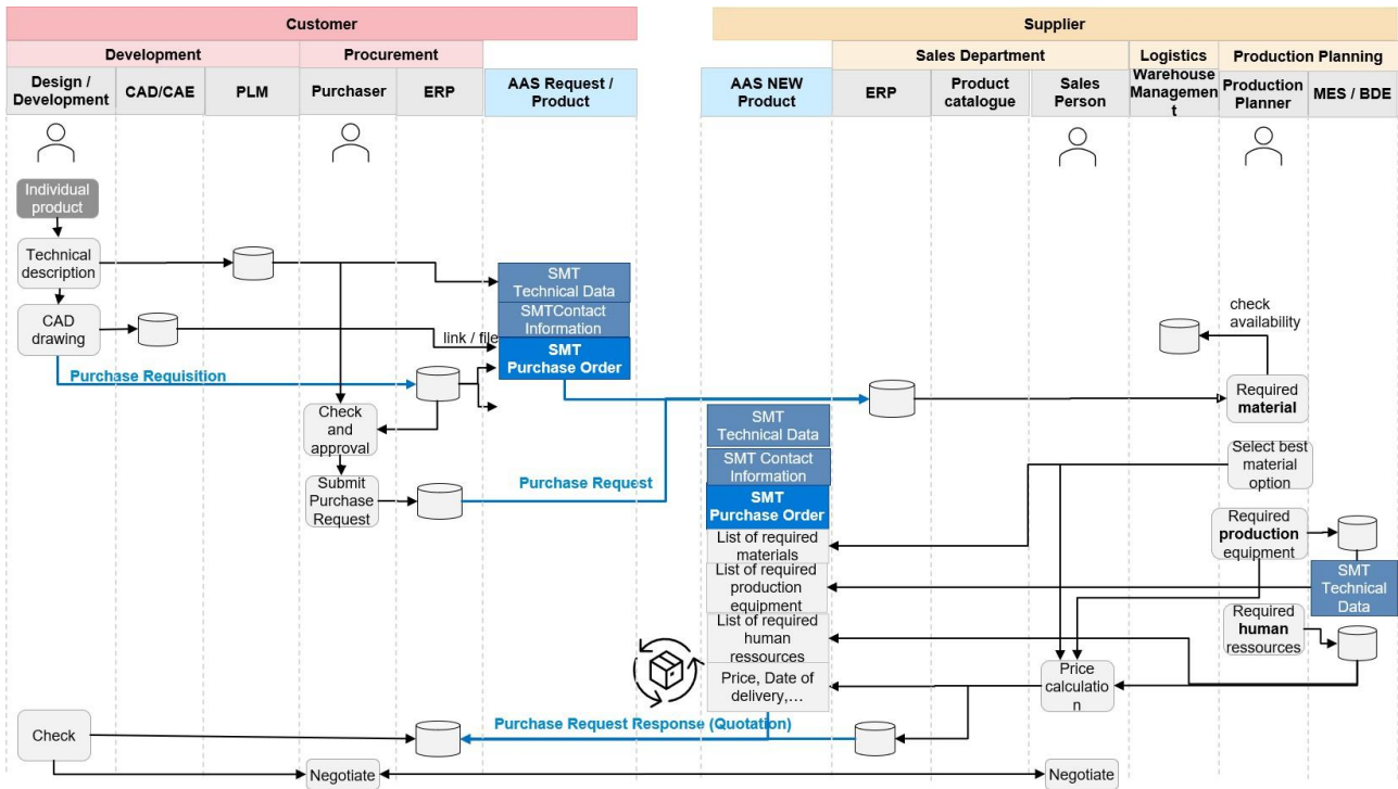
Figure 5. Purchase request process for individual / not existing products (Scenario 3)
