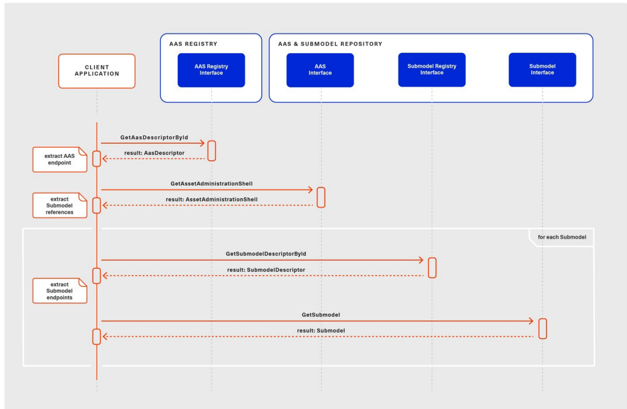
Figure 9 Interaction for Client Application using AAS and Submodel Interfaces (included Submodel Registry)
