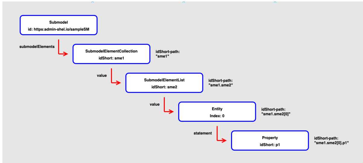
Figure 6 Example Hierarchy of Submodel Elements
