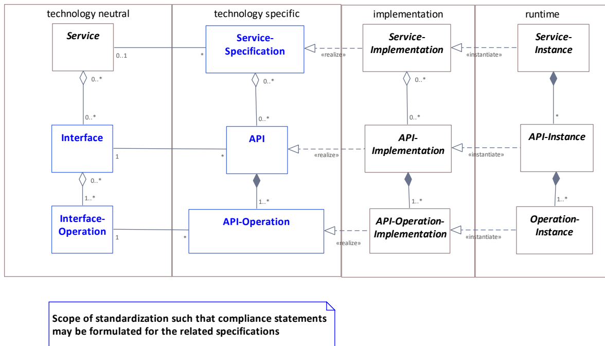
Figure 2 Services, Interfaces & APIs and Operations
