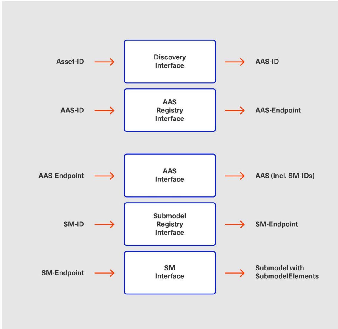
Figure 3 Retrieval of Asset-related Information by AAS and Submodels
