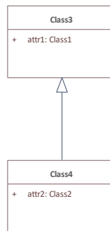
Figure 21 Inheritance/Generalization
