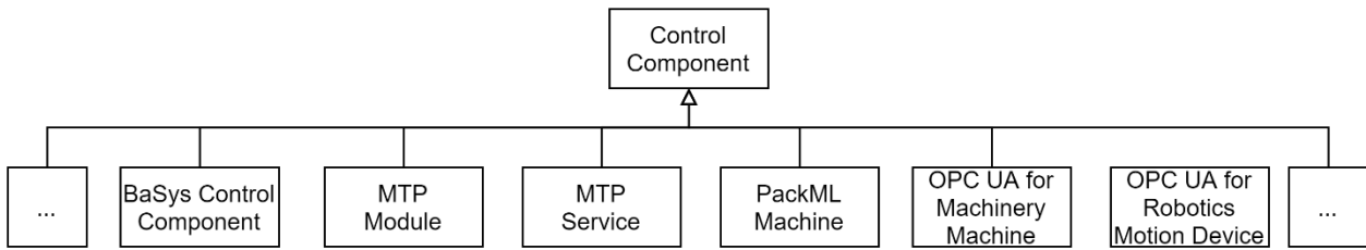
Figure 1: Using Control Components as Abstract Asset Type
