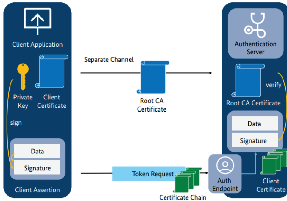
Figure 5 The private_key_certchain_jwt method [...download service]
