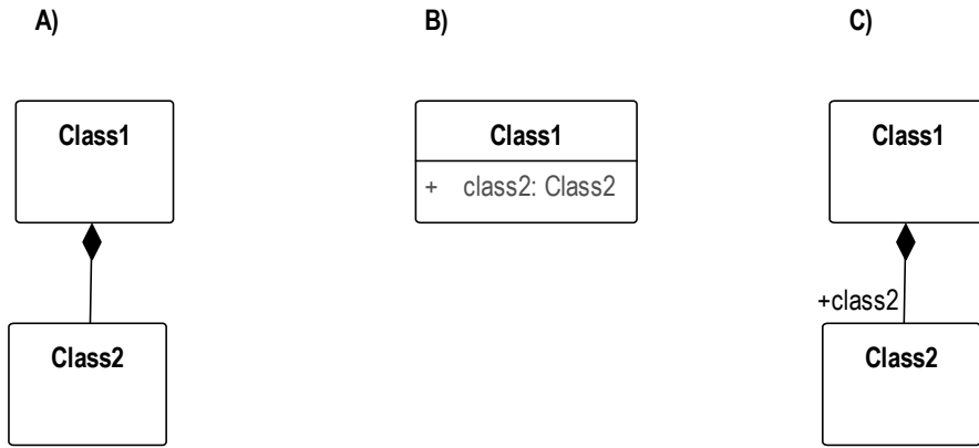
Figure 23 Graphical Representations of Composite Aggregation/Composition
