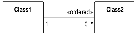
Figure 9 Ordered Multiplicity
