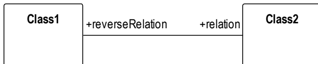
Figure 10 Association
