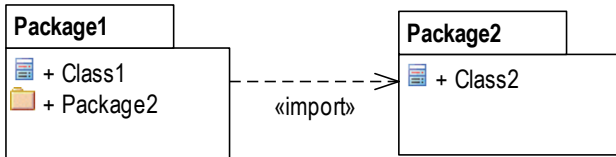
Figure 17 Imported Package
