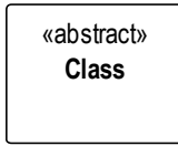
Figure 15 Abstract Class
