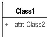
Figure 6 Class
