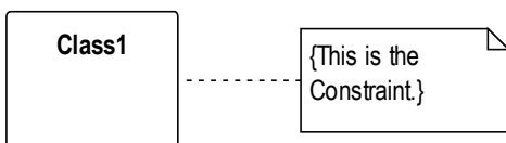
Figure 22 Constraint
