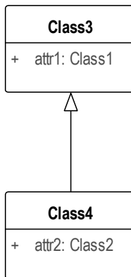
Figure 7 Inheritance/Generalization
