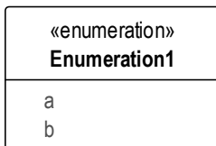
Figure 18 Enumeration
