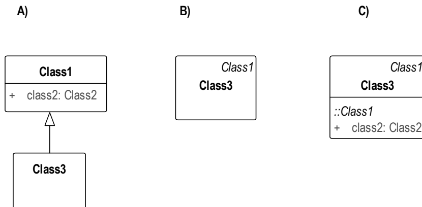
Figure 25 Graphical Representation of Generalization/Inheritance
