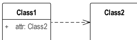
Figure 14 Dependency
